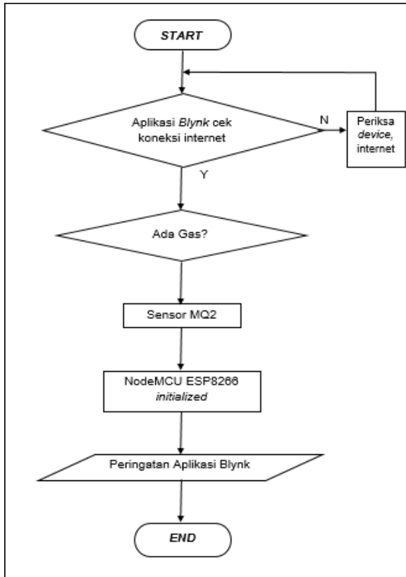
Gambar 4. Flowchart Kontrol Kebocoran Gas
