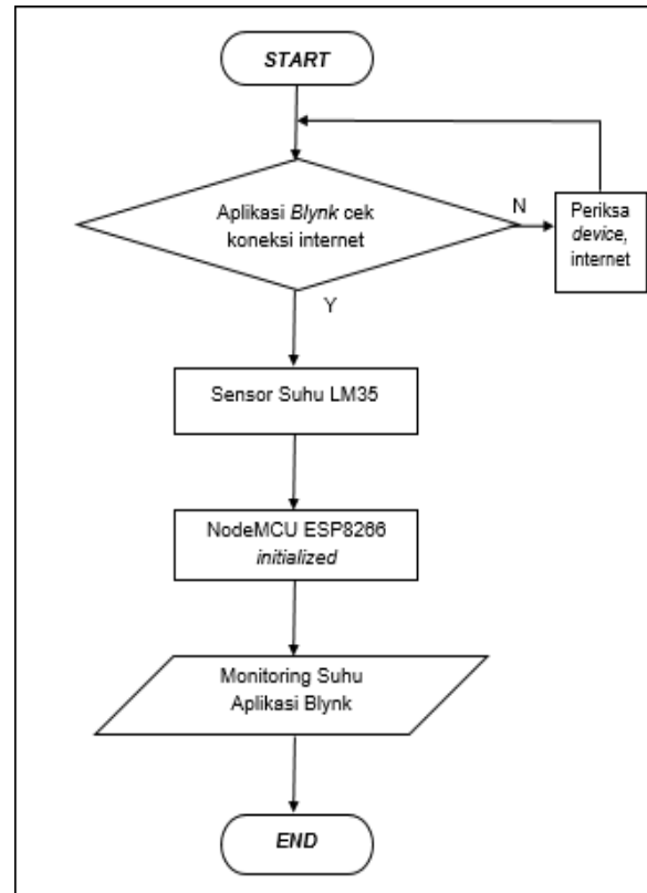
Gambar 5. Flowchart Kontrol Suhu
